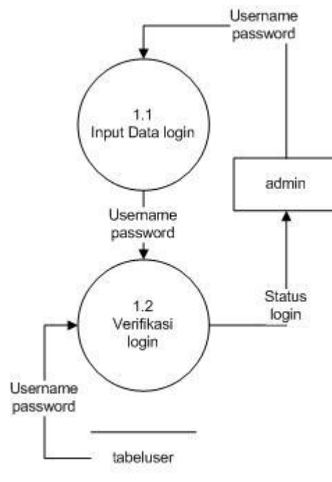
Gambar 3.3 DFD Level 2 Proses Login
